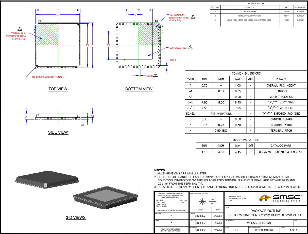
Figure 2 LPC47N217N 56-Pin QFN Package, 8x8mm Body, 0.5mm Pitch
